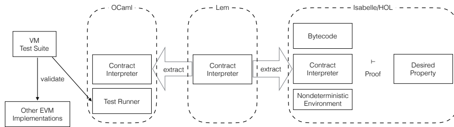
Fig. 3. Our Lem definition can be extracted into OCaml and Isabelle/HOL. We tested the OCaml extraction against the standard VM test suite. Using the Isabelle/HOL extraction, we proved safety properties about some bytecodes. In this figure, the VM test suite and other EVM implementations are not our contributions.
